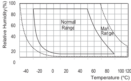
Figure 4. Operating Conditions
