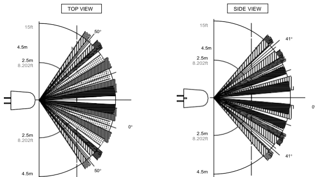
The X-Y cross-sectional diagram shows the detection area.
